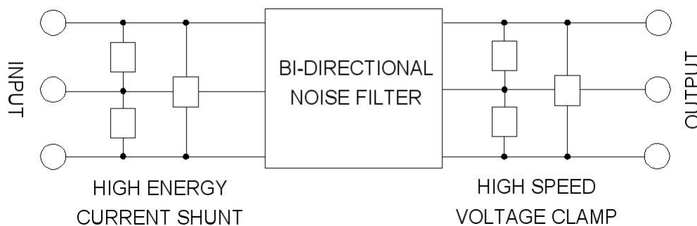
SSP20 Block Diagram
